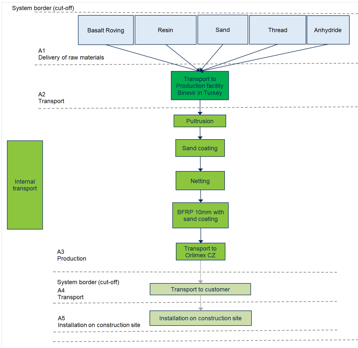
LCA process diagram according to EN 15804 (7.2.1)
